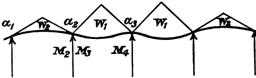
FIG. 151.—Continuous beam with triangular distribution of load.
