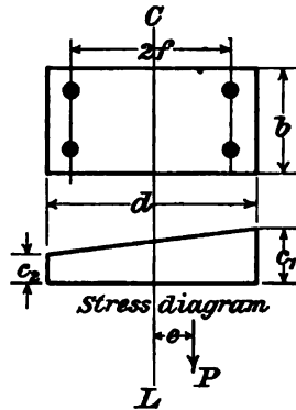
FIG. 30.—Rectangular section symmetrically reinforced under bending and direct compression.
