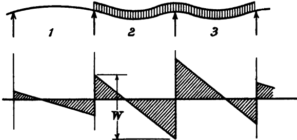
FIG. 83.—Shearing force diagram.
