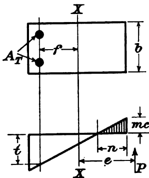
FIG. 31.—Bending and compression, P falling outside d .
