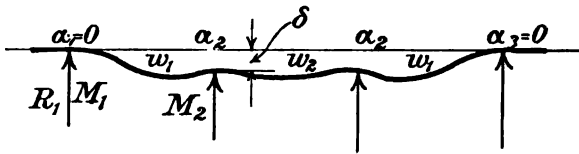
FIG. 157.—Effect of settlement on beam of many spans.
