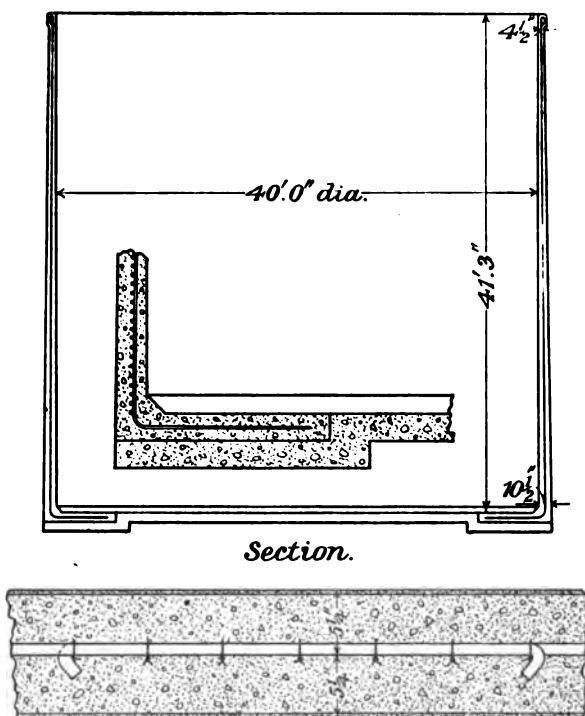
FIG. 119.—Detail of reservoir at Mittagong, N.S.W.
