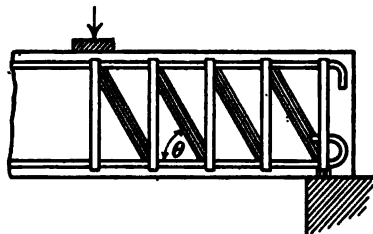
FIG. 51.—Shearing resistance of beams with stirrups.
