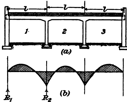
FIG. 65 (a) and (b).—Three spans equally loaded.
