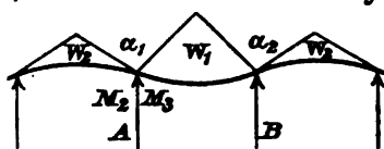
FIG. 150.—Continuous beam with triangular distribution of loads.
