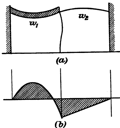
FIG. 69 (a) and (b).—Two spans, one loaded.
