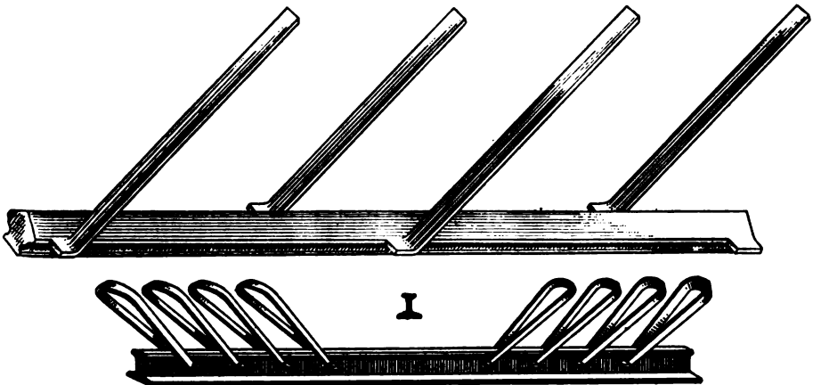
FIG. 5.—Types of patent bars designed to give increased shear resistance.
