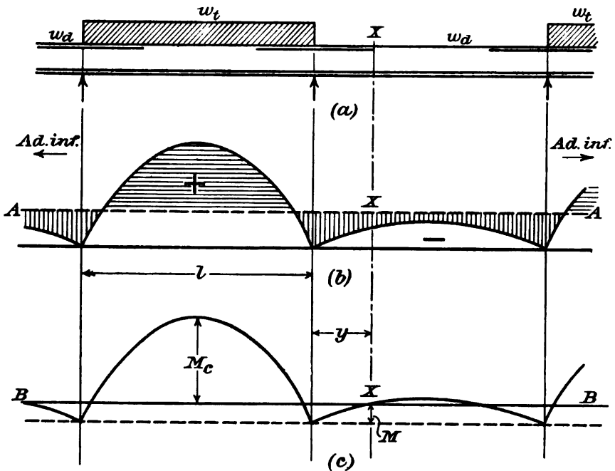
FIG. 109.—Bending moments on slabs.
