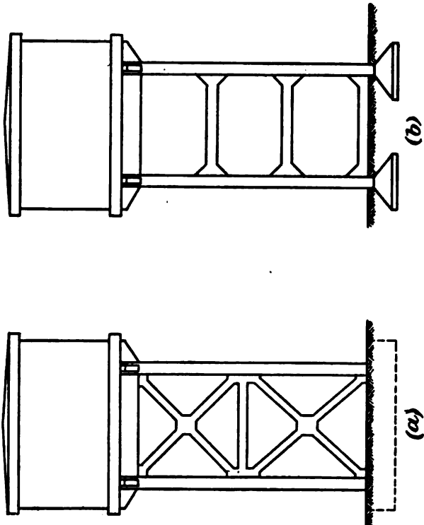
FIG. 121.—Bracing of columns of water tower.
