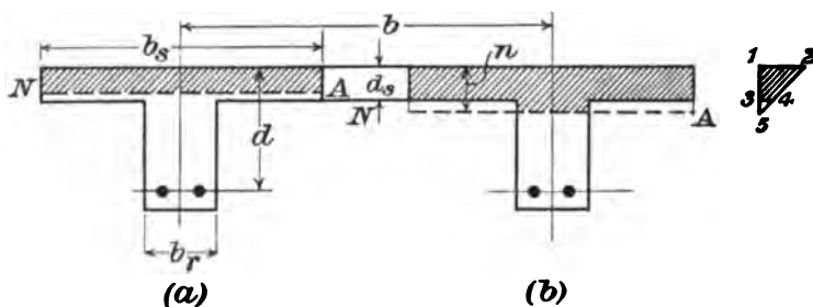
FIG. 17.—Cross-section through T-beam.
